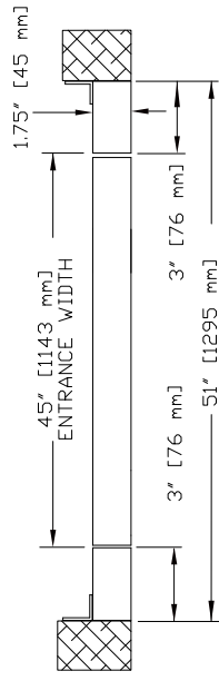
HORIZONTAL SECTION
