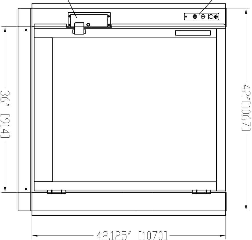
FRONT VIEW (33.25" [845mm] CLEAR OPENING)
