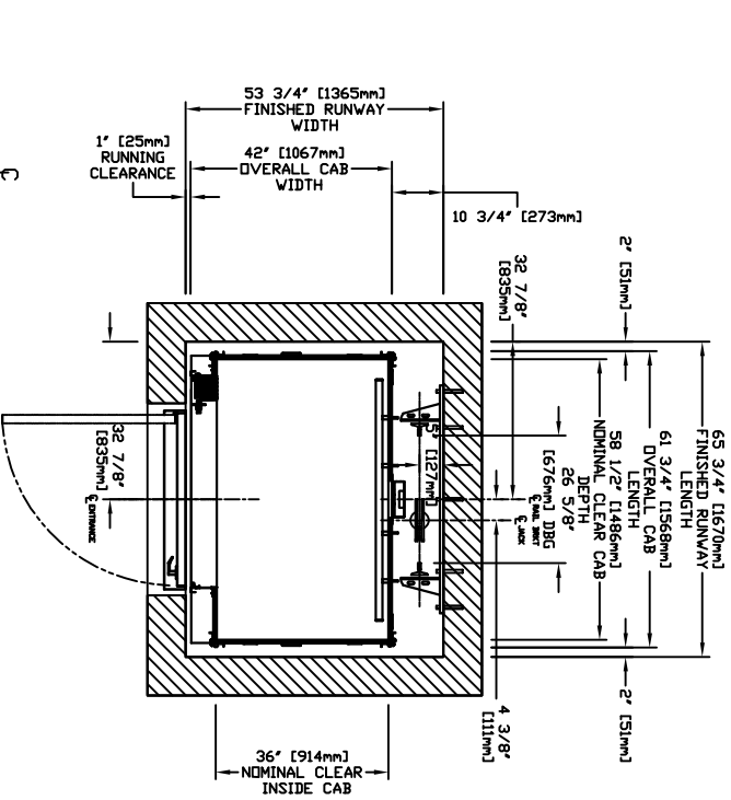
PLAN VIEW - INFINITY Model 3660 TYPE 5
