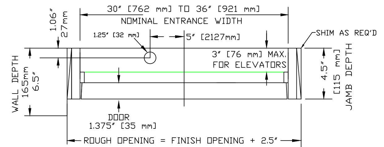
HORIZONTAL SECTION
