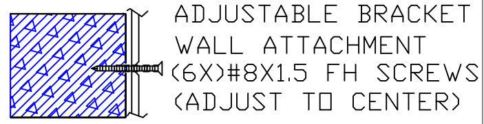
HORIZONTAL SECTION
