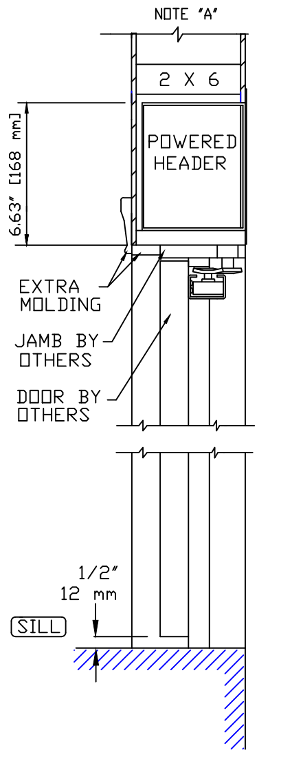
VERTICAL SECTION
