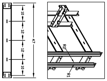
RAIL BRACKETS
